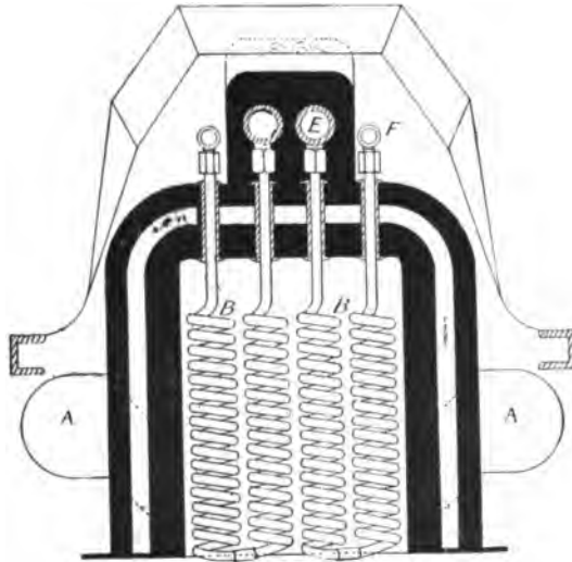
FIG. 181.—Front Elevation of the Flash Generator of the Automobile Manufacturing Co., of England. A A are spaces for side draughts; B B, flash tubes; E, steam chamber; F, water feed pipes. The whole is covered by such a "bonnet" as is familiar on large gasoline cars.
